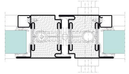
Janisol C4 EI60/EI90 EI60 / EI90
